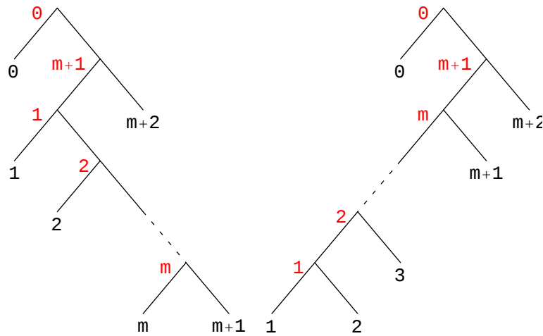
FIGURE 6. Tree pair diagram (T_-, T_+) for the word x_1^m x_m^{-1} x_{m-1}^{-1} \cdots x_1^{-1} with the carets and the leaves numbered.
